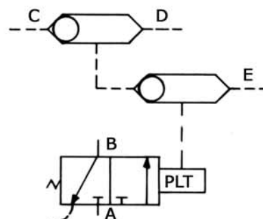
OR Circuit
